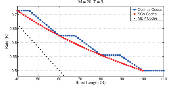
Fig. 4. Achievable rates for different code constructions for burst lengths B from 40 to 110 and delay of T = 5 macro packets with each having M = 20 channel packets.
