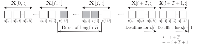
Fig. 2. Channel Model. The erasure burst spans a total of B channel packets as shown. Each source packet \mathbf{s}[i] arrives just before the transmission of \mathbf{X}[i, :] and needs to be reconstructed by the destination after a delay of T macro-packets.
