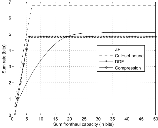
Fig. 2. Sum rate comparison of the zero-forcing, DDF, and compression strategies, along with the cut-set outer bound. Note that the DDF and generalized compression strategies are evaluated under their respective distributions that achieve to within a constant gap to capacity for each strategy. In particular, they are not evaluated under their respective optimal distributions, so the numerical result does not imply that the compression strategy outperforms DDF.
