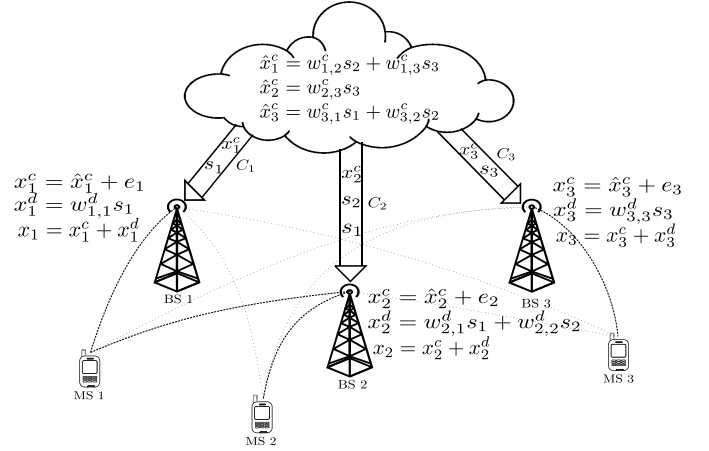
Fig. 7. The hybrid data-sharing and compression strategy for the downlink C-RAN.
