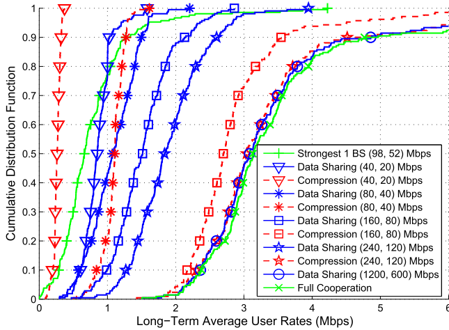
Fig. 3. Cumulative distribution function of user rates for the data-sharing and compression strategies with adaptive quantization and single antenna terminals for varying fronthaul/backhaul capacities.
