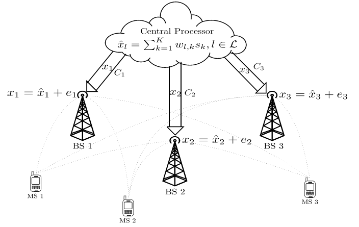
Fig. 2. The compression strategy for the downlink C-RAN.
