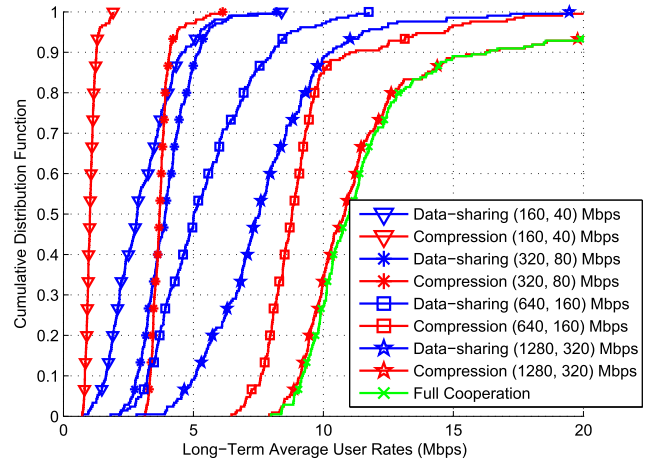
Fig. 4. Cumulative distribution functions of user rates for the data-sharing and compression strategies with fixed quantization and multi-antenna terminals for varying fronthaul/backhaul capacities.
