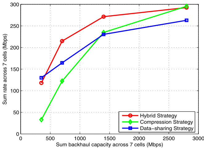
Fig. 8. Comparison of the hybrid strategy with the data-sharing and compression strategies.
