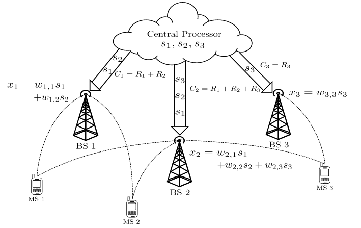
Fig. 1. The data-sharing strategy for the downlink C-RAN.
