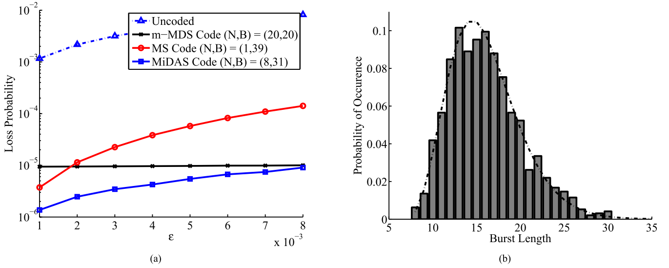
Fig. 20. Simulation Experiments for Fritchman Channel Model with (\mathcal{N}, \alpha, \beta) = (8, 10^{-5}, 0.5) . (a) Simulation over a \mathcal{N} + 1 = 9 -States Fritchman Channel with (\alpha, \beta) = (10^{-5}, 0.5) . All codes are evaluated using a decoding delay of T = 40 packets and a rate of R = 40/79 \approx 0.5 . (b) The actual burst histogram (in bars) follows a negative binomial distribution (dotted line) with \mathcal{N} = 8 failures and a success probability of \beta = 0.5 .
