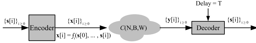
Fig. 2. The source stream \mathbf{s}[t] for t \geq 0 is causally encoded to a channel stream \mathbf{x}[t] which is transmitted over the sliding window erasure channel \mathcal{C}(N, B, W) . The decoder tolerates a maximum delay of T packets.
