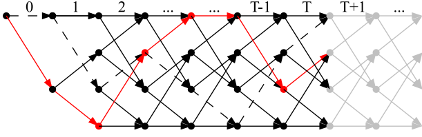
Fig. 25. Trellis diagram showing a streaming code. Since the delay constraint is T packets, the corresponding generator matrix is truncated at time T (cf. (74)) and hence nodes after time T are irrelevant. Also, according to the column distance and column span definitions in Def. 3 and Def. 4, only paths diverging from all zero path at the starting point are considered to calculate these metrics. The red solid path is one example of these paths while the dashed line is not considered.
