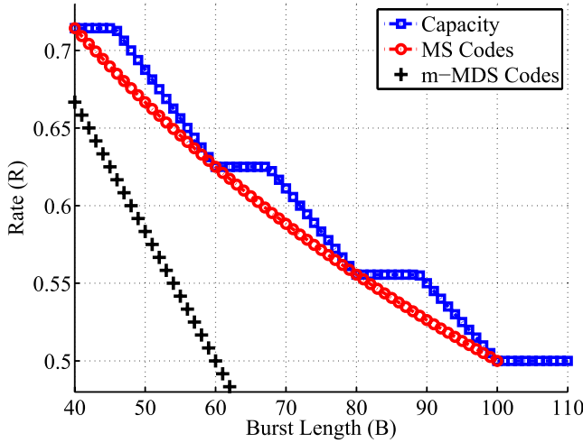
Fig. 6. Achievable rates for different code constructions for the case of unequal source-channel inter-arrival rates for the \mathcal{C}(N = 1, B, W = M(T+1)) channel. We fix the delay to T = 5 macro-packets and let M = 20 . The blue plot (marked with squares) corresponds to the capacity in Theorem 3. The red curve (marked with circles) corresponds to the rate achieved by the adapted MS code (18) whereas the black line corresponds to the rate of the m -MDS code (16).
