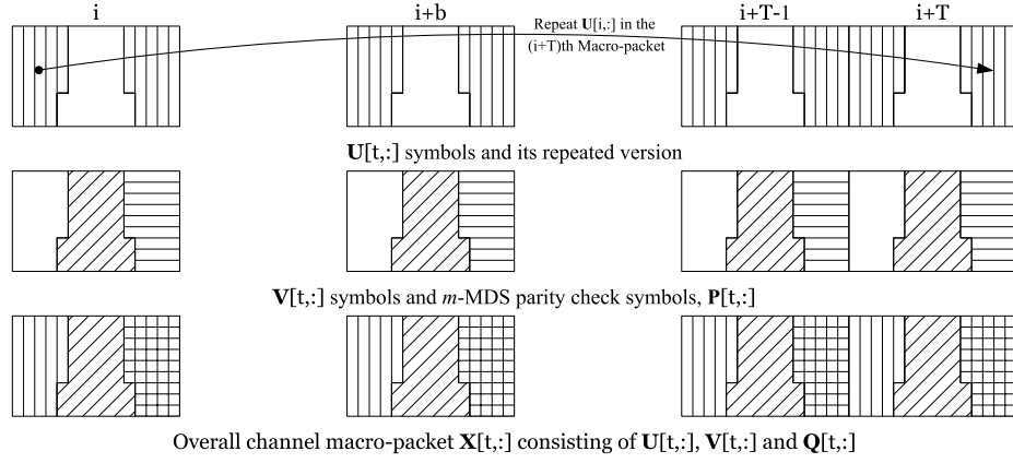
Fig. 13. Encoding of source packets into macro-packets. Each source packet is split into two groups. A repetition code is applied to the U[t, :] group with a delay of T macro-packets and is denoted by vertically hatched boxes as shown in the first figure. A m -MDS code is applied to the V[t, :] group which is denoted by diagonally hatched boxes to generate the parity-checks P[i, :] denoted by the horizontally hatched boxes as shown in the second figure. The combination of the resulting parity-checks of the two groups is indicated in the last figure with grid hatched boxes.
