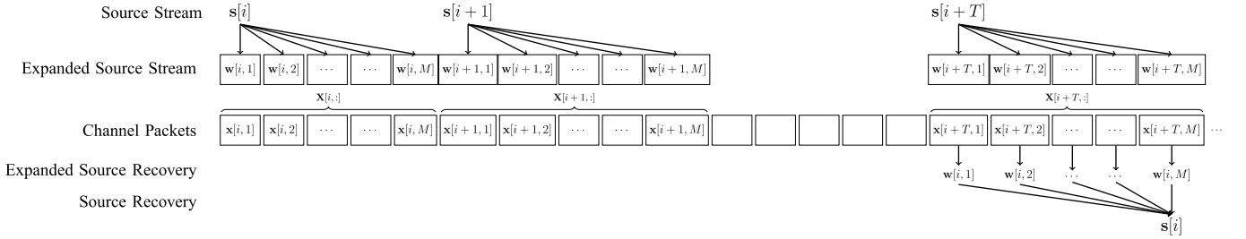
Fig. 4. Each source symbol s[i] is split into M sub-packets i.e., s[i] = (w[i, 1], w[i, 2], \dots, w[i, M]) . The expanded source stream is then encoded using a Maximally-Short code. The decoder recovers each w[i, j] once y[i + T, j] is received which ensures that s[i] is recovered by the end of the macro-packet i + T .
