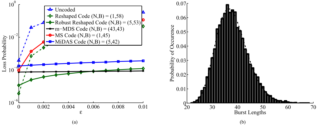
Fig. 24. Simulation Experiments for Fritchman Channel Model with \mathcal{N} + 1 = 20 states and (\alpha, \beta) = (10^{-5}, 0.5) . (a) Simulation results. All codes are evaluated using a decoding delay of T = 2 macro-packets and a rate of R \approx 0.63 . Each macro-packet consists of M = 40 channel packets. (b) The actual burst histogram (in bars) follows a negative binomial distribution (dotted line) with \mathcal{N} = 20 failures and a success probability of \beta = 0.5 .
