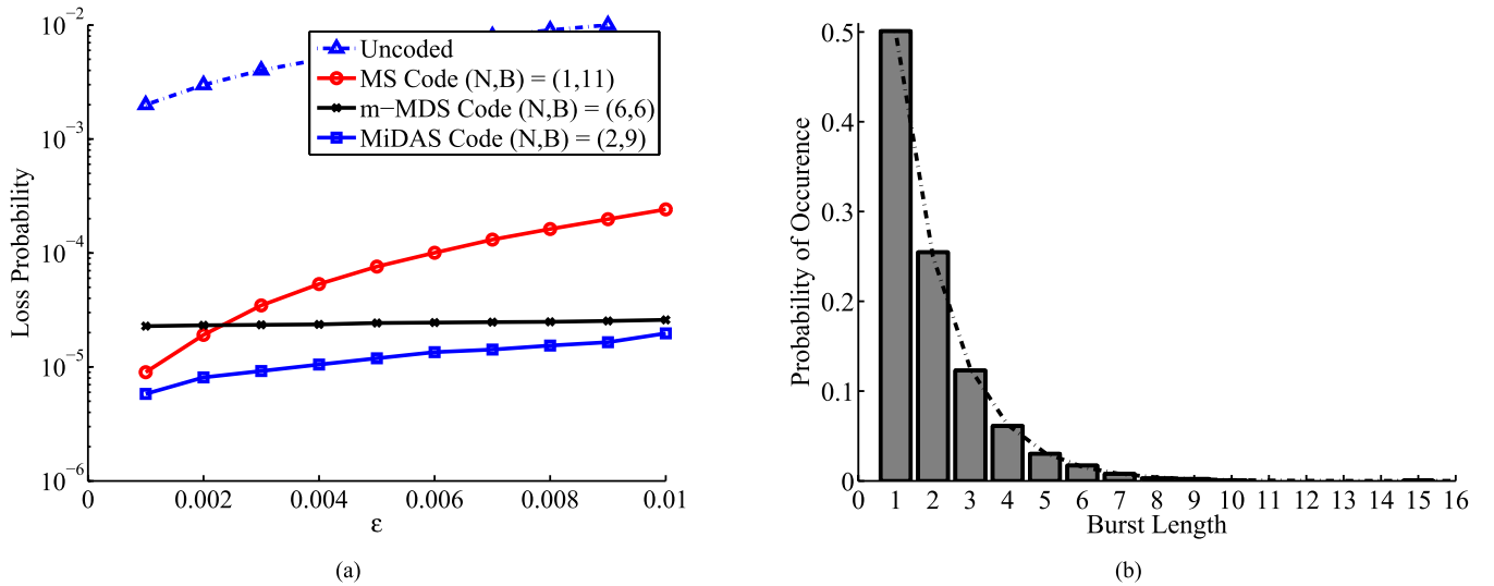
Fig. 18. Simulation Experiments for Gilbert-Elliott Channel Model with (\alpha, \beta) = (5 \times 10^{-4}, 0.5) . (a) Simulation results. All codes are evaluated using a decoding delay of T = 12 packets and a rate of R = 12/23 \approx 0.52 . (b) The actual burst histogram (in bars) follows a geometric distribution (dotted line) with a success probability of \beta = 0.5 .
