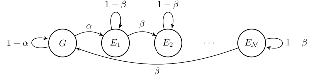
Fig. 17. Fritchman Channel Model.
