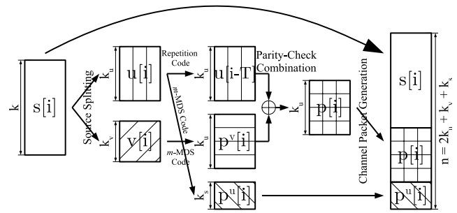
Fig. 9. A block diagram illustrating the encoding steps of a MiDAS code. The top part is equivalent to that of a Generalized MS code (cf. Fig. 8). The lower part shows the extra layer of parity-checks added which is generated by applying a m -MDS code to the \mathbf{u}[\cdot] sub-packets.
