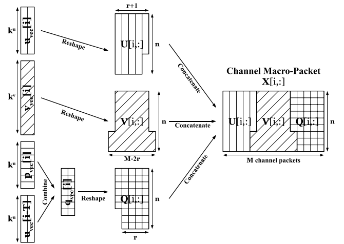
Fig. 12. Reshaping of Channel Packets. The three groups, u_{\text{vec}}[i] , v_{\text{vec}}[i] and q_{\text{vec}}[i] are reshaped into \mathbf{U}[i, :] , \mathbf{V}[i, :] and \mathbf{Q}[i, :] which are denoted by vertically, diagonally and grid hatched boxes, respectively. These reshaped packets are then concatenated to form the channel macro-packet \mathbf{X}[i, :] .
