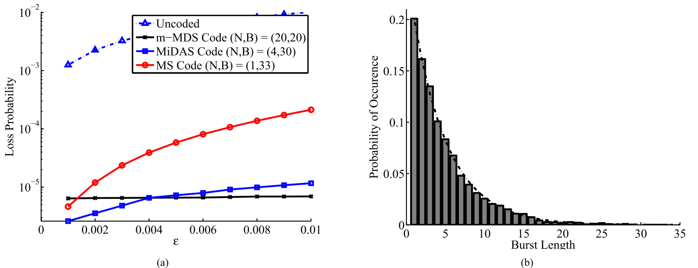
Fig. 19. Simulation Experiments for Gilbert-Elliott Channel Model with (\alpha, \beta) = (5 \times 10^{-5}, 0.2) . (a) Simulation results. All codes are evaluated using a decoding delay of T = 50 packets and a rate of R = 50/83 \approx 0.6 . (b) The actual burst histogram (in bars) follows a geometric distribution (dotted line) with a success probability of \beta = 0.2 .
