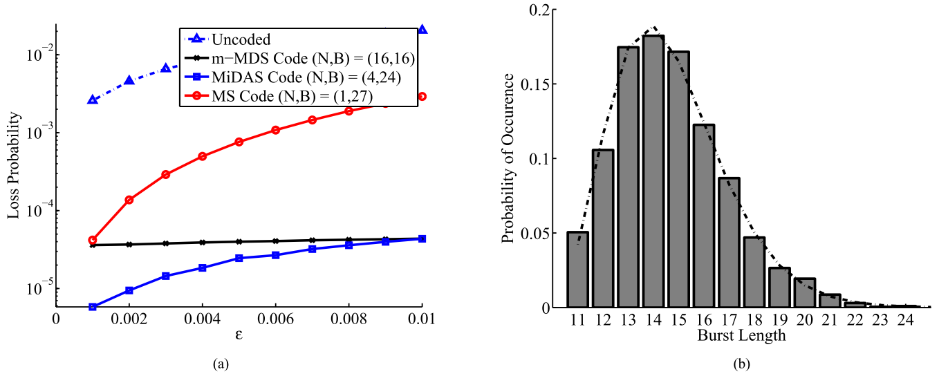
Fig. 21. Simulation Experiments for Fritchman Channel Model with (\mathcal{N}, \alpha, \beta) = (11, 2 \times 10^{-5}, 0.75) . (a) Simulation over a \mathcal{N} + 1 = 12 -States Fritchman Channel with (\alpha, \beta) = (2 \times 10^{-5}, 0.75) . All codes are evaluated using a decoding delay of T = 40 packets and a rate of R = 40/67 \approx 0.6 . (b) The actual burst histogram (in bars) follows a negative binomial distribution (dotted line) with \mathcal{N} = 11 failures and a success probability of \beta = 0.75 .
