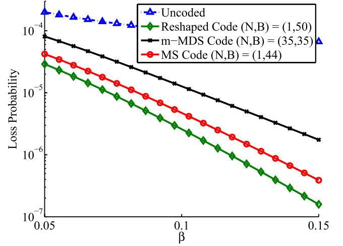
Fig. 23. Simulation over a Gilbert Channel with \alpha = 10^{-5} and \beta varied on the x-axis. All codes are of rate R = \frac{9}{14} and evaluated using a decoding delay of T = 4 macro-packets. Each macro-packet consists of M = 20 channel packets.
