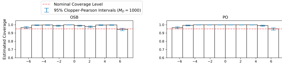
Figure 5. (Left) OSB 95% interval coverage. (Right) PO 95% interval coverage using a flat prior mean constructed from the mean of the true bin expectations. Both methods construct intervals with at least nominal coverage.
