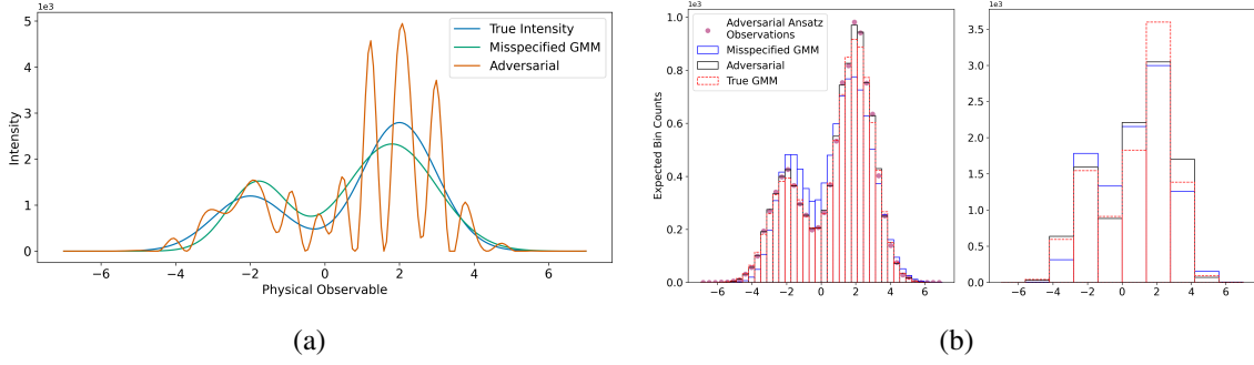
Figure 1. (a): illustration of the true intensity function used for simulations and the two ansatz functions used for computing the smearing matrix \mathbf{K} . (b): (Left) True bin expected counts. The deviations in each bin between the true expectation and the ansatz expectations drives the systematic error. (Right) Smeared bin expected counts. Note the reduced magnitude of difference in expectation with respect to the true space, emphasizing the convolutional nature of the smearing matrix.
