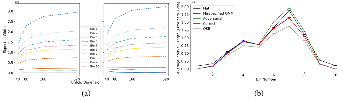
Figure 11. (a): estimated expected 95% interval widths as a function of the number of true unfolding bins provide assurance that both OSB and PO intervals remain finite as the number of true bins increases. Both OSB (Left) and PO (Right) interval widths become less sensitive to unfolding dimension as the number of true bins increases. (b): the choice of prior used when optimizing 95% PO interval does not have a substantial impact on the expected interval widths. We observe that for three incorrectly specified priors (Flat, Misspecified GMM, and Adversarial), in all but three bins, the expected interval widths are close. In bins 6, 7, and 8, we observe the width benefits of having a more correctly specified prior. We also observe the closeness of most bin expected interval widths to the expected OSB interval widths.
