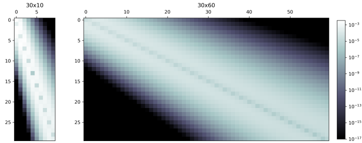
Figure 13. |K_{ij} - K_{ij}^{\text{MC}}| for all rows i and columns j for the (left) 30 \times 10 and (right) 30 \times 60 matrices. The misspecification in the 30 \times 10 case is O(10^2) times larger than that of the 30 \times 60 case.
