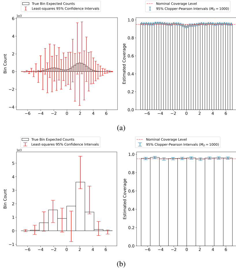
Figure 3. (a): unfolding with n = 40 true bins and least-squares intervals. The Left and Right are analogous to those in figure 2, but with the n = 40 true bins. Using more true bins fixes the coverage problem of the least-squares intervals in figure 2 ( Right ), at the expense of significantly wider bin-wise intervals. (b): ( Left ) Bin count intervals from one out of the M samples using post-inversion aggregation with the Misspecified GMM Ansatz. ( Right ) Estimated bin-wise coverage of the post-inversion aggregation approach shows these intervals have the desired coverage.
